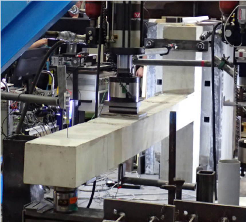
Figure 2 - Test arrangement
