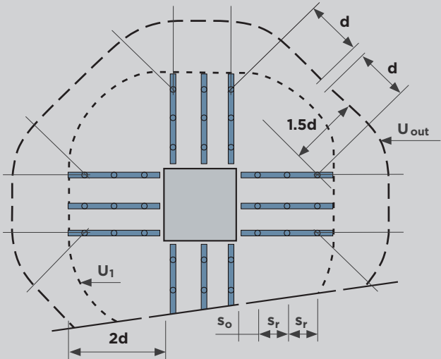
Figure 3 Detailing requirements
